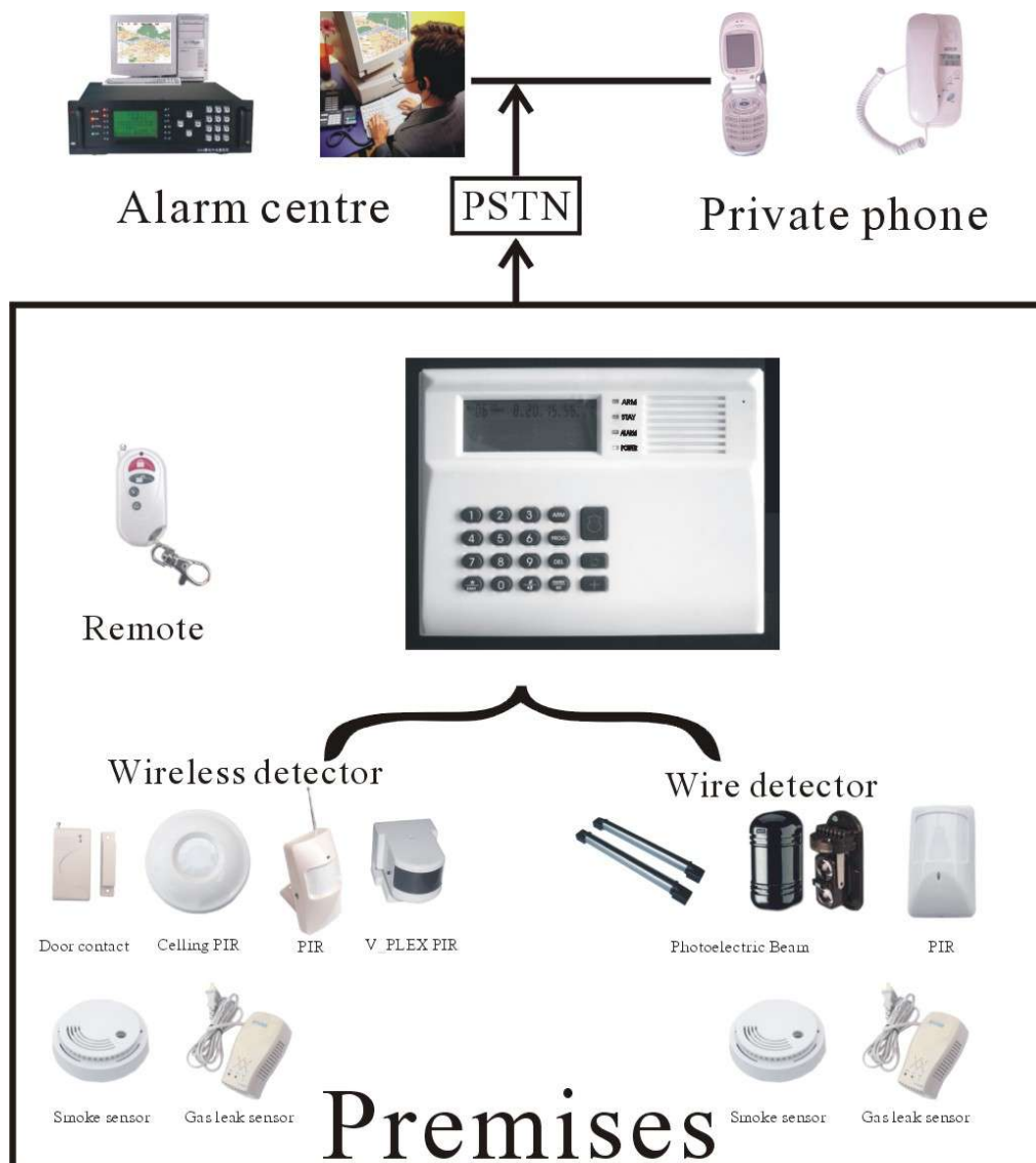
Figure 1: Basic principle of operation
